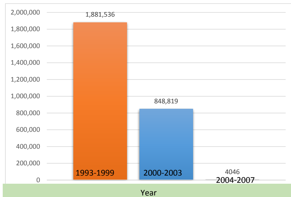
Figure 2. 18: Trend Analysis for POP-PBDE composition in EEE
