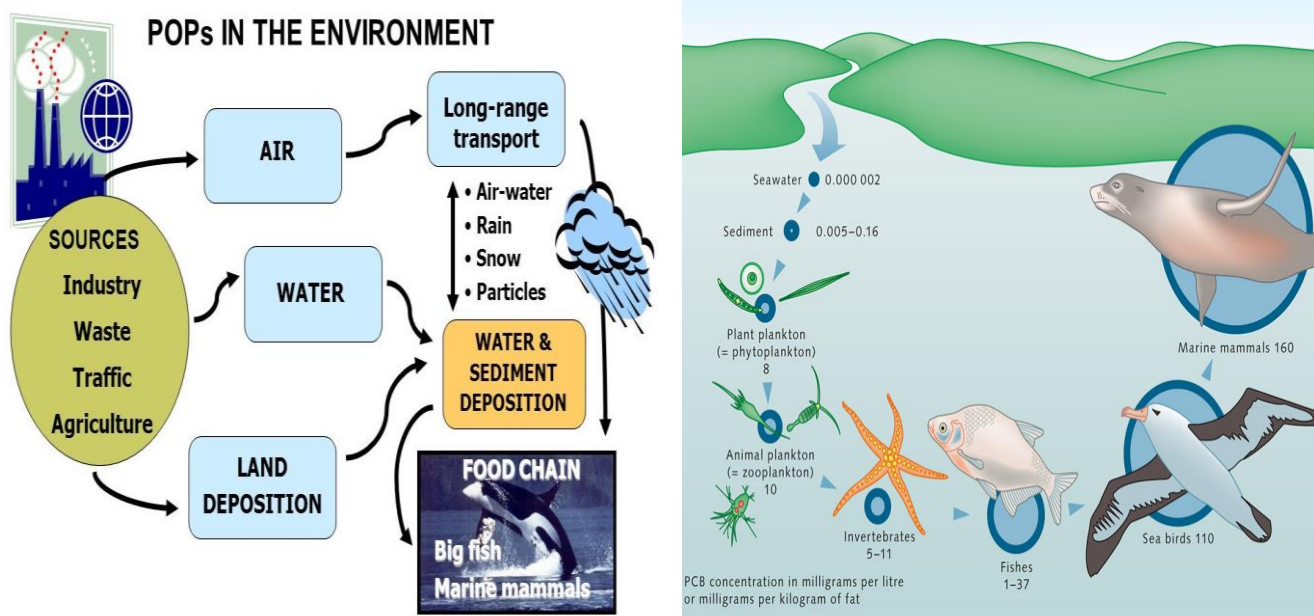
Figure 1. 1: POPs transportation, accumulation and magnification in the environment. Sources: WHO (2011), World Ocean Review (2015)
